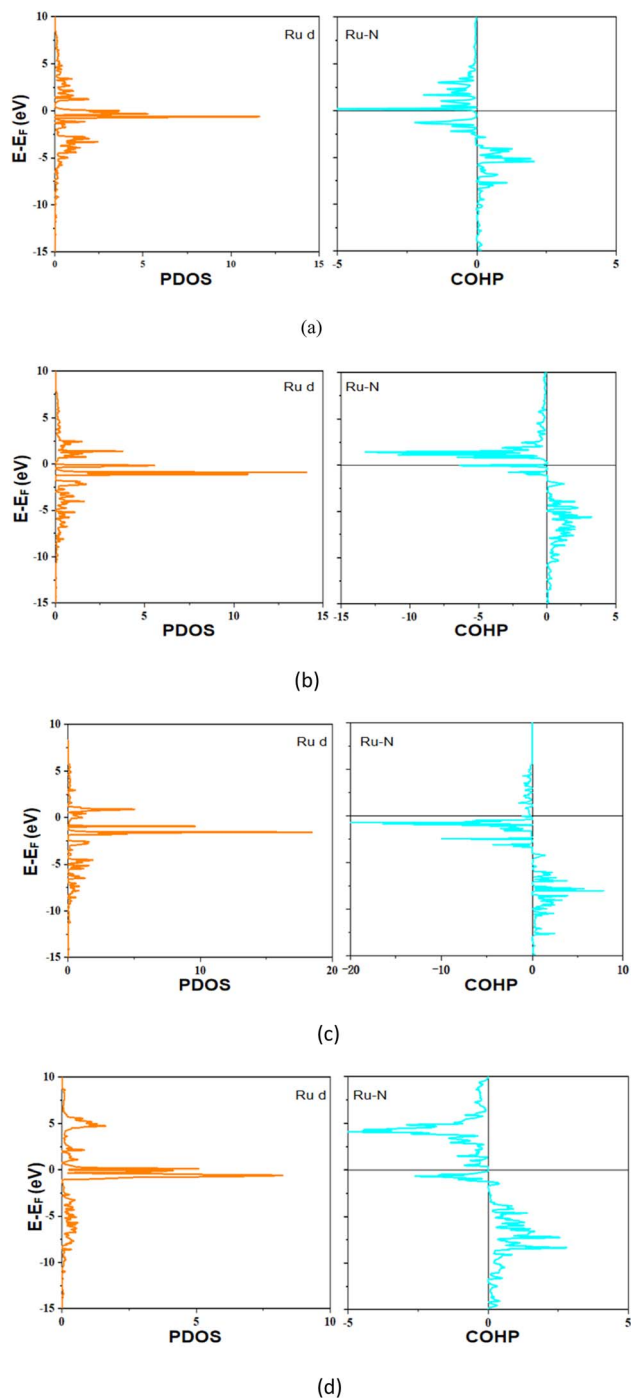
Fig. 4 Calculated PDOS and COHP analysis for Ru SACs on the (a) N_{\text{pyrrolic}} , (b) 2N, (c) 3N and (d) 4N-doped graphene substrates.
