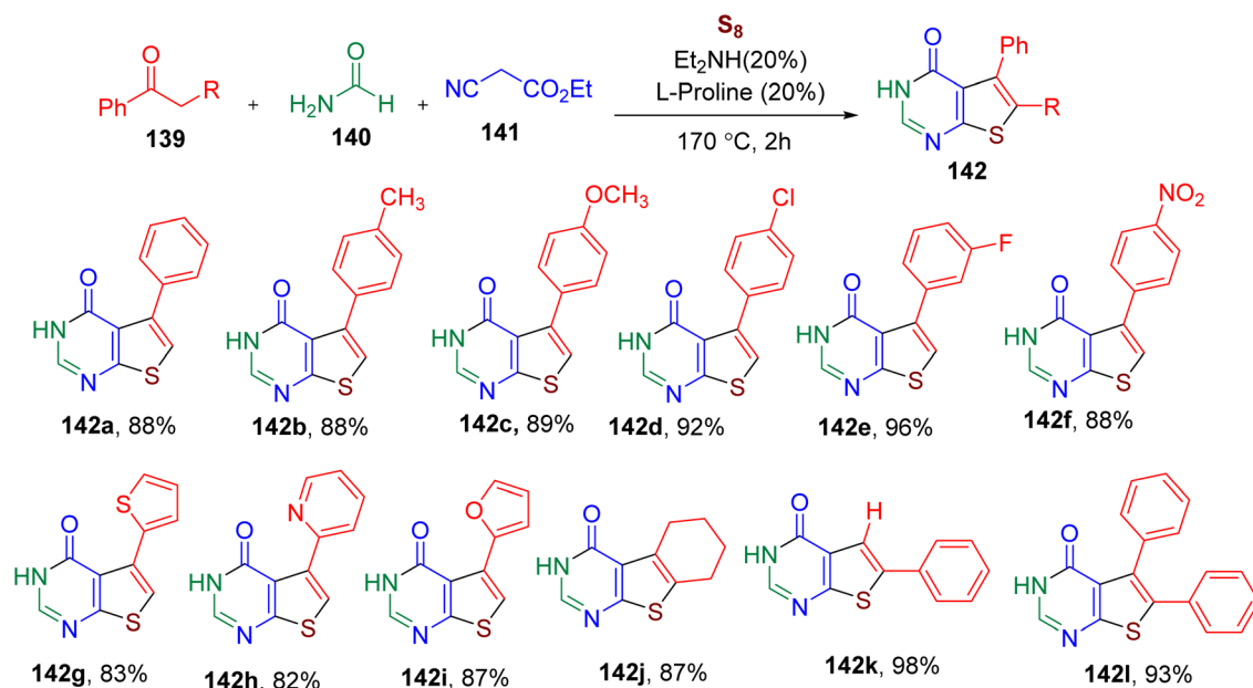
Fig. 36 MCR for the synthesis of thieno[2,3- d ]pyrimidin-4(3 H )-ones.
