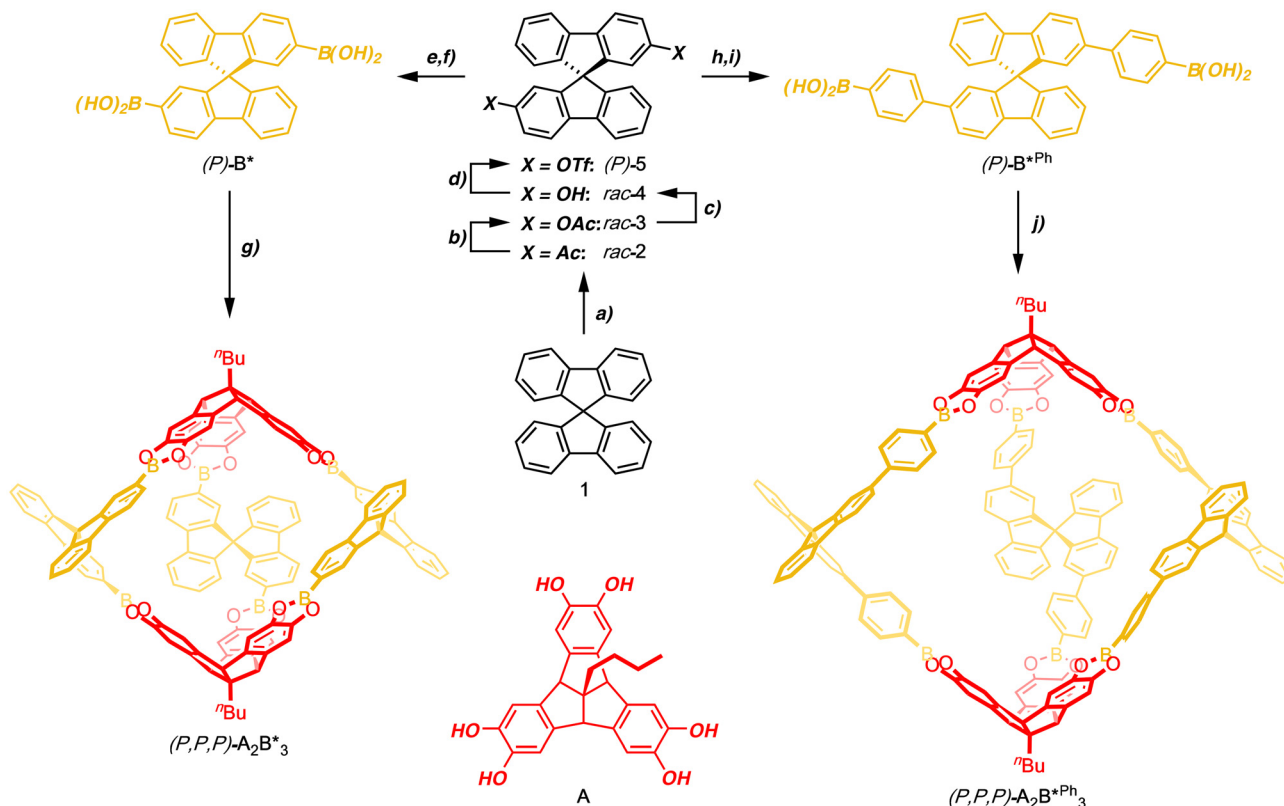
Scheme 1 Synthesis of chiral linkers and cages: (a) \text{AlCl}_3/\text{CH}_2\text{Cl}_2/\text{MeNO}_2 1 : 1, rt, 12 h, 96%; 53 (b) m\text{CPBA} , \text{CH}_2\text{Cl}_2 , 45 °C, 2 d, 73%; 54,55 (c) \text{NaOH}/\text{H}_2\text{O} , \text{MeOH} , 50 °C, 10 min, 96%; 54 (d) 1. HPLC separation; 53 2. \text{TF}_2\text{O}/\text{NEt}_3 , \text{CH}_2\text{Cl}_2 , -78 °C, 2 h, 73%; 55 (e) \text{Pd}(\text{OAc})_2/\text{XPhos}/\text{KOAc}/\text{B}_2\text{pin}_2 , 1,4-dioxane, 110 °C, 1 d, 99%; 55 (f) \text{MeB}(\text{OH})_2/\text{TFA} , \text{CH}_2\text{Cl}_2 , rt, 1 d, (P): 72%, rac: 68%; (g) A , 4 Å MS, THF, rt, 5 d, 74%; (h) \text{Pd}(\text{OAc})_2/\text{SPhos}/\text{K}_3\text{PO}_4/4\text{-TMSPb}(\text{OH})_2 , 1,4-dioxane/ \text{H}_2\text{O} 5 : 1, 100 °C, 1 d, 93%; (i) \text{BBr}_3 , \text{CH}_2\text{Cl}_2 , rt, 2 h, (P): 98%, rac: 67%; (j) A , 4 Å MS, THF, rt, 14 d, 65%.
