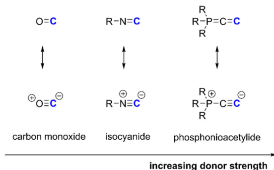
Fig. 1 Selection of sp-hybridized neutral carbon ligands and their resonance structures.
