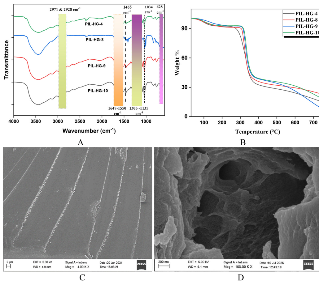
Fig. 1 (A) FT-IR overlay, (B) TGA curve overlay of poly(ionic liquid) based hydrogels with different crosslinker ratios, and (C) & (D) FE-SEM images of PIL-HG-8 .
