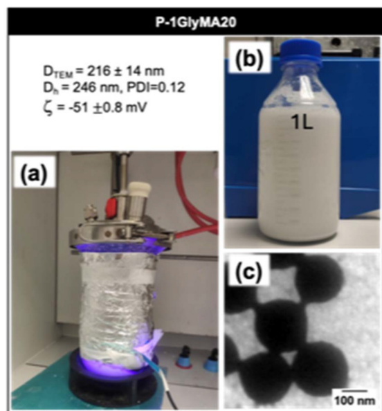
Fig. 7 Scale-up of surfactant-free latex synthesis via photo-SFEP of GlyMA under 405 nm irradiation. (a) Reaction setup for the scale-up to 1 liter, using R = 1\text{‰} and SC = 20\% w/w. (b) The resulting stable latex dispersion produced in a 1 L batch. (c) TEM image of nanoparticles in the latex.
