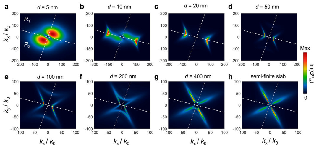
Fig. 6 The distribution of the imaginary part of reflected Green's function in momentum space, \text{Im}(\mathbf{G}_{zz}^R(k_x, k_y)) for different thicknesses of bGO slab. The frequency is fixed to 718 \text{ cm}^{-1} . The white dashed lines are parallel to the effective optic axes, dividing the k space into four quadrants.
