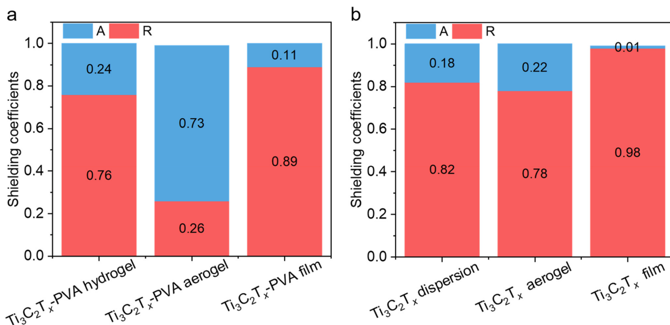
Fig. 5 Absorption coefficient (A) and reflection coefficient (R) of the (a) Ti_3C_2T_x -PVA-based hydrogel, aerogel, and film and (b) Ti_3C_2T_x -based dispersion, aerogel, and film at a fixed Ti_3C_2T_x areal density ( 20 \text{ mg cm}^{-2} ).
