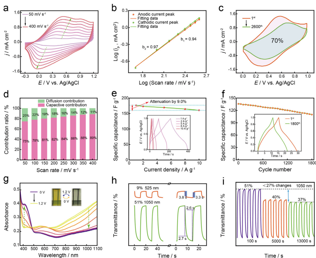
Fig. 3 Electrochemical properties of PHTPA . (a) The CVs of PHTPA in the BFEF system (scan rate range: 50–400 \text{mV s}^{-1} , voltage interval: −0.3–1.2 V). (b) The b value was obtained by fitting the peak currents of the cathode and anode with the voltage. (c) PHTPA CV stability (at 100 \text{mV s}^{-1} ). (d) Pseudocapacitance contribution ratio of PHTPA (scan rate range: 50–400 \text{mV s}^{-1} ). (e) Rate performance of the PHTPA film, with the inset showing capacitance values at different current densities. (f) Capacitive stability of the PHTPA film (at 10 \text{A g}^{-1} ). (g) Spectroelectrochemical curves of PHTPA films (voltage interval: 0–1.2 V). (h) Transmittance values and response times of PHTPA films at 525 nm and 1050 nm. (i) Transmittance stability of PHTPA films at 1050 nm.
