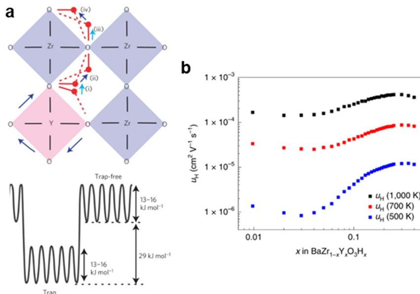
Fig. 9 (a) Proton transport steps and the corresponding energies. This figure has been adapted from ref. 121 with permission from Springer Nature, copyright 2025. (b) Proton mobility in Ba(Zr, Y)O 3-δ at 500, 700 and 1000 K. A low Y doping level reduces the proton mobility. This figure has been adapted from ref. 125 with permission from Springer Nature, copyright 2025.
