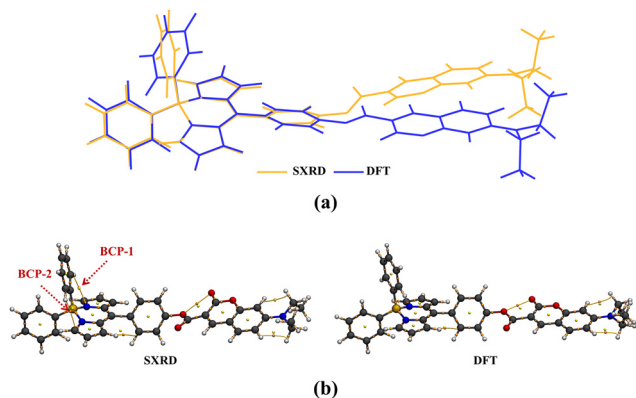
Fig. 3 (a) Overlay of DFT-computed conformations for FMR-I (M06-2X/6-31+G** in vacuum), with a ‘relaxed’ single-crystal X-ray diffraction (SXR D) conformation in orange (hydrogen and disordered heavier atoms optimized) and a freely-optimized conformation in blue. (b) Molecular graphs for both conformers with bond critical points (3, -1 ) in orange and ring critical points (3, +1 ) in yellow.
