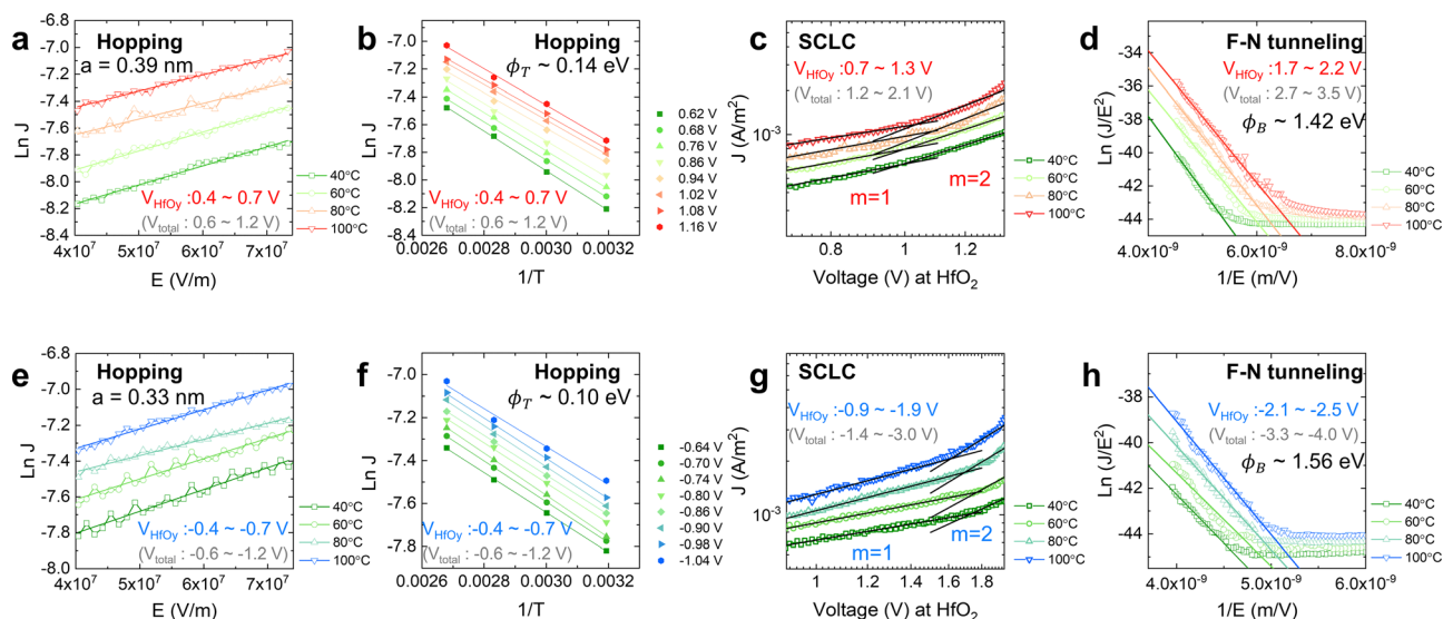
Fig. 4 (a) Hopping conduction in the \text{HfO}_2 layer (0.6 V to 1.2 V). (b) Arrhenius plots for the \text{HfO}_2 layer. (c) Double logarithmic I - V curves of the THT memristor in the positive region, showing ohmic ( m = 1 ) and space-charge-limited conduction ( m = 2 ) behavior (1.2 V to 2.1 V). (d) F-N tunneling in the \text{HfO}_2 layer (2.7 V to 3.5 V). (e) Hopping conduction in the \text{HfO}_2 layer (−0.6 V to −1.2 V). (f) Arrhenius plots for the \text{HfO}_2 layer. (g) Double logarithmic I - V curves of the THT memristor in the negative region (−1.4 V to −3.0 V). (h) F-N tunneling in the \text{HfO}_2 layer (−3.3 V to −4.0 V).
