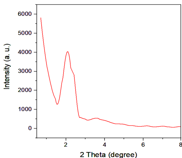
Fig. 3 Low-angle PXRD pattern of \text{Fe}_3\text{O}_4 @MCM-41@UiO-66/SB-Pd.
