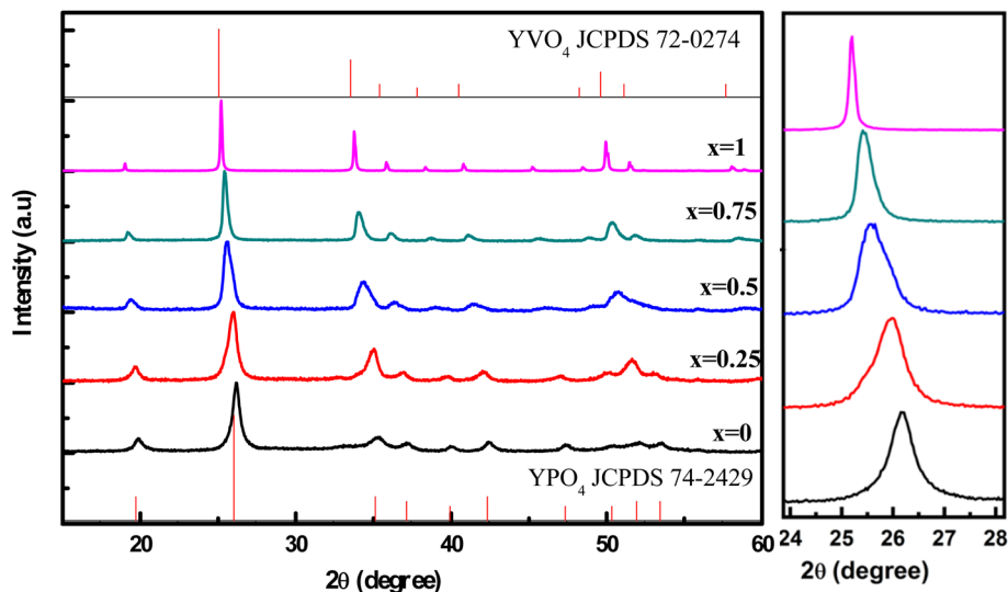
Fig. 1 XRD patterns of YP_{(1-x)}V_xO_4:5\% \text{ Eu} materials ( x = 0, 0.25, 0.50, 0.75 , and 1 ).
