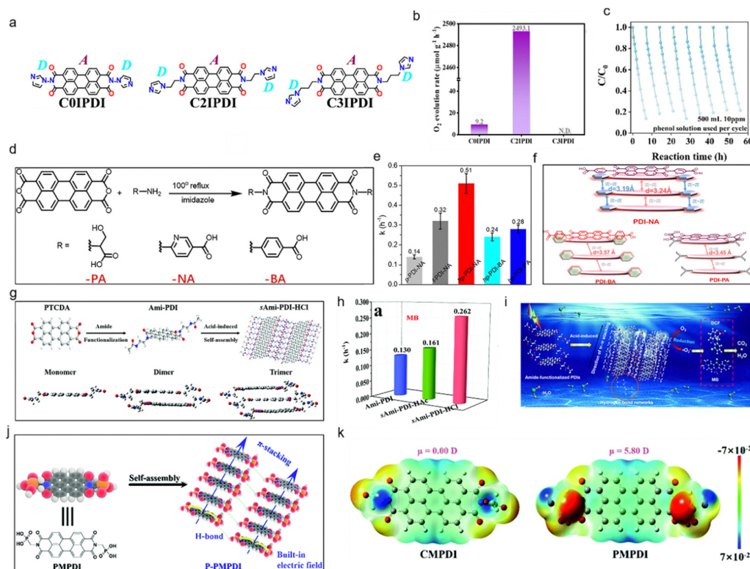
Fig. 2 (a) Different \sigma lengths of molecular structures about C n IPDI. (b) Comparison of photocatalytic O 2 evolution rate on C n IPDI. (c) Cyclic stability of C2IPDI. Reproduced from ref. 56. Copyright 2023, Wiley. (d) The synthesis method of PDI-NA molecular and reference catalyst. (e) TOC removal rate and mineralization rate constant over different photocatalysts. (f) A schematic diagram of PDI-NA, PDI-BA and PDI-PA. Reproduced from ref. 33. Copyright 2022, Elsevier. (g) The synthesis process and structure of sAmi-PDI-HCl (over) and the DFT calculations regarding geometries of sAmi-PDI-HCl monomers, dimers, and trimers (below). (h) The kinetics constants toward MB. (i) The mechanism for photocatalytic degradation process when using amide-functionalized supramolecular PDI. Reproduced from ref. 30 Copyright 2020, the Royal Society of Chemistry. (j) The synthesis of supramolecular P-PMPDI. (k) Diagram of molecular dipoles and electron distribution in PDI derivatives. Reproduced from ref. 62. Copyright 2019, the Royal Society of Chemistry.
