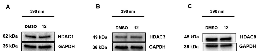
Fig. 5 Immunoblot analysis of HDAC isoform levels in MM1.S cells after irradiation with 390 nm. MM1.S cells were treated with 12 (1 \mu M) or vehicle (DMSO) for 6 h. HDAC1 (A), HDAC3 (B), and HDAC8 (C) levels were analyzed by immunoblotting. GAPDH was used as loading control. Representative images from a total of n = 2 replicates.
