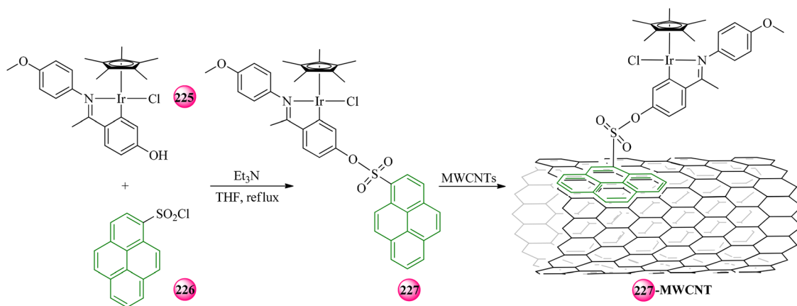
Fig. 66 The synthesis procedure for the immobilization of iridacycle 227 onto MWCNTs. Reproduced with permission from ref. 8 Copyright 2017, American Chemical Society.
