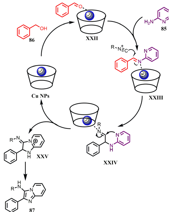
Fig. 9 Plausible mechanism for synthesis of N -(alkyl)-2-phenylimidazo[1,2- a ]pyridin-3-amine derivatives using \text{Cu}@\beta\text{-CD}@\text{MGO} nanoparticles.
