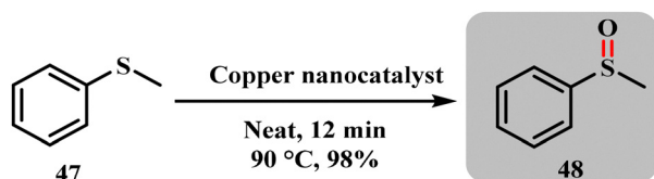
Scheme 22 \text{Cu(II)} catalysed oxidation of sulphides into sulphoxides (Heidari et al. ).
