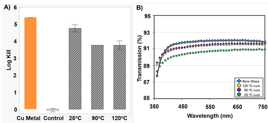
Fig. 7 Antimicrobial efficacy and optical transmission results for Ferro 221 glass coatings dosed with copper glass-ceramic (CGC) powder extracts with triethyl phosphite (TEP) ( [Cu]_{Tot} = 600 ppm) and cured at different temperatures. A. Average log-kill values against S. aureus for various coating cure conditions. Control sample has no antimicrobial additive. Error bars represent the standard deviation of duplicate samples. B. Optical transmission measurements.
