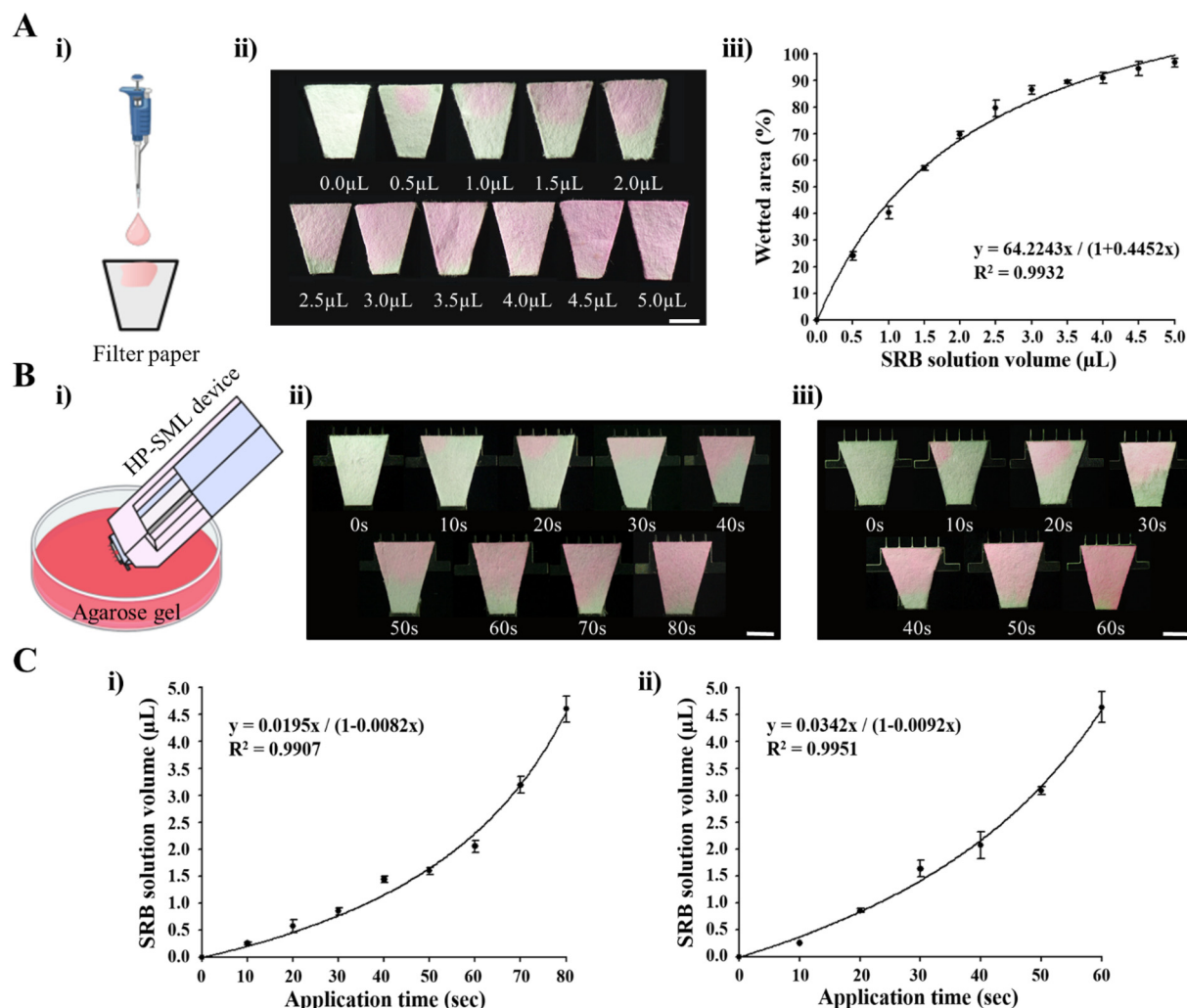
Fig. 4 Quantification of ISF absorbed by filter paper attached to the HP-SML device. (A) Schematic illustration (i) of the addition of SRB solution (0 to 5 μL with 0.5 μL intervals) to the filter paper using a micropipette and an optical image of the wetted filter papers with SRB solutions (ii) (scale bar = 3 mm). Graph and trend formula describing the relationship between the wetted area of the filter paper on the MN and the volume of the SRB solution (iii). (B) Schematic diagram (i) of the application of the HP-SML device to papers with SRB solutions (ii) (scale bar = 3 mm). Graph and trend formula describing the relationship between the wetted area of agarose gel containing SRB for different times (0–80 s at 10 s intervals) and optical images of filter papers when the HP-SML device with a 750 μm MN (ii) and 1400 μm MN (iii) was used (scale bars = 3 mm). (C) Graph and trend line showing the relationship between the application time of the HP-SML device and the volume of SRB solution extracted by the HP-SML device with a 750 μm MN (i) and 1400 μm MN (ii). All the schematics were created using BioRender.
