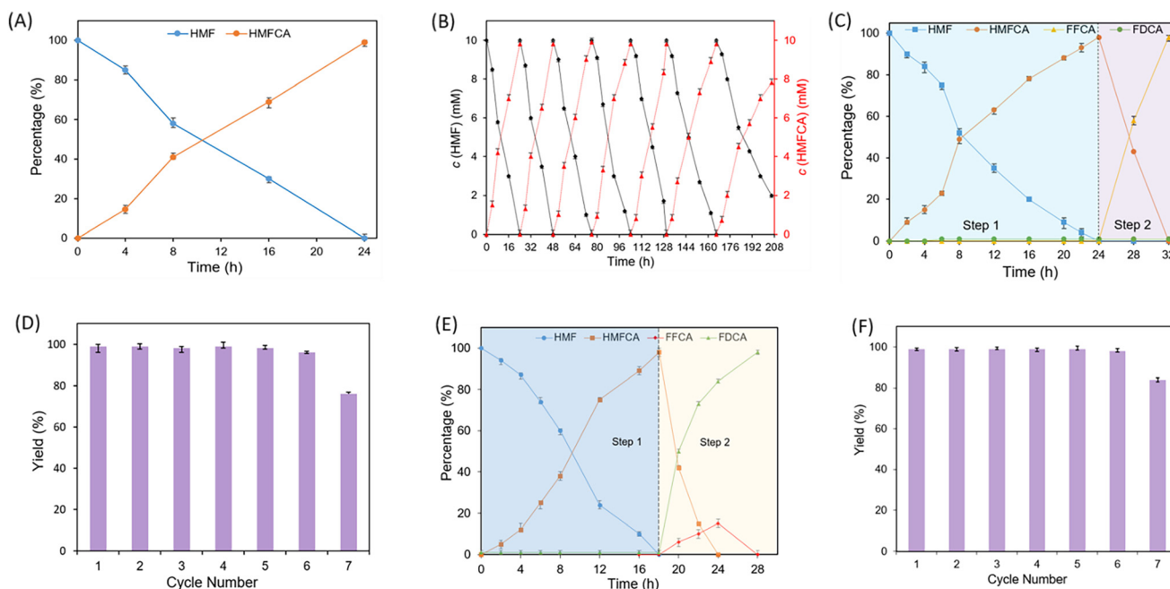
Fig. 4 The immobilized enzymes selectively oxidized HMF to produce HMFFCA, FFCA and FDCA. (A and B) For HMFFCA. Reaction conditions: 0.1 mM NAD + , 0.02 mM NFCM, 10 mM HMF, 0.08 or 0.16 μM HLADH and 0.1 or 0.2 μM rAaeUPO were added into 2 mL of phosphate buffer (50 mM, pH 7.0) in turn. (C and D) For FFCA. After HMF was completely transformed, HLADH and rAaeUPO were taken out and 2 μM GOase was added, and the mixture was shaken at 30 °C (300 rpm). (E and F) For FDCA. Reaction conditions: 0.24 μM HLADH and 0.3 μM rAaeUPO were used. Percentage (%) is the ratio of the concentration of each component in the mixture and calculated according to the formula given in section 1.8 in the ESI†.
