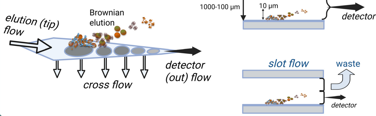
Fig. 2 Schematic of major separation processes and fluxes operations associated with asymmetric flow field-flow fractionation.
