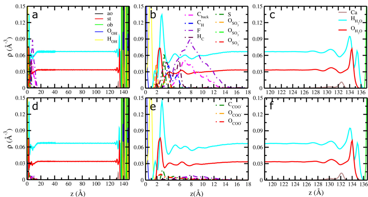
Fig. 1 Computed atomic density profiles (ADPs) of PFAS and H 2 O molecules in Ca-kaolinite as a function of the distance normal to the basal hydroxyl surface. (a–c) 6:2 FTS (d–f) 6:2 FTC. H 2 O (solid yellow) and O OH (solid blue) represent the ‘H’ and ‘O’ atoms of the hydroxyl groups in kaolinite, respectively. The O H 2 O and H H 2 O are shown as solid red and cyan. Dashed lines represent the atoms of the 6:2 FTS/6:2 FTC molecules. The O SO 3 and S SO 3 represent oxygen and sulfur atoms in 6:2 FTS and the O COO and C COO represent oxygen and carboxyl carbon atoms in 6:2 FTS. The C back , F and H c corresponds to carbon backbone, fluorine and hydrogens in each FT’s. Labels – ao, st, and ob represent surface atoms in kaolinite following the notation used in clayff. 55 The origin ( z = 0 ) is the mean position of the basal ‘O’ atoms at the hydroxyl surface of kaolinite.
