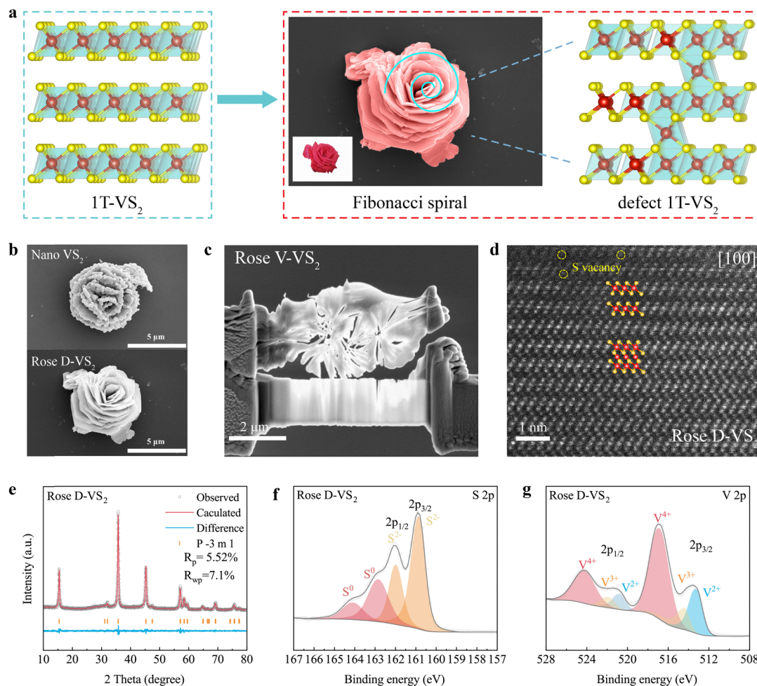
Fig. 1 Structure and morphology characterization of the Rose D-VS 2 . (a) Design concept of defect-rich VS 2 micro-rose materials. Inset: The optical photograph of a rose. (b) SEM images illustrating the morphological evolution process of the Rose D-VS 2 . (c) Cross-section SEM image showing the morphology of the Rose D-VS 2 . (d) The HADDF-STEM image revealing the atomic structure of the Rose D-VS 2 . (e) Rietveld refinement of the XRD pattern of the Rose D-VS 2 . (f) High-resolution V 2p XPS spectrum of the Rose D-VS 2 . (g) High-resolution S 2p XPS spectrum of the Rose D-VS 2 .
