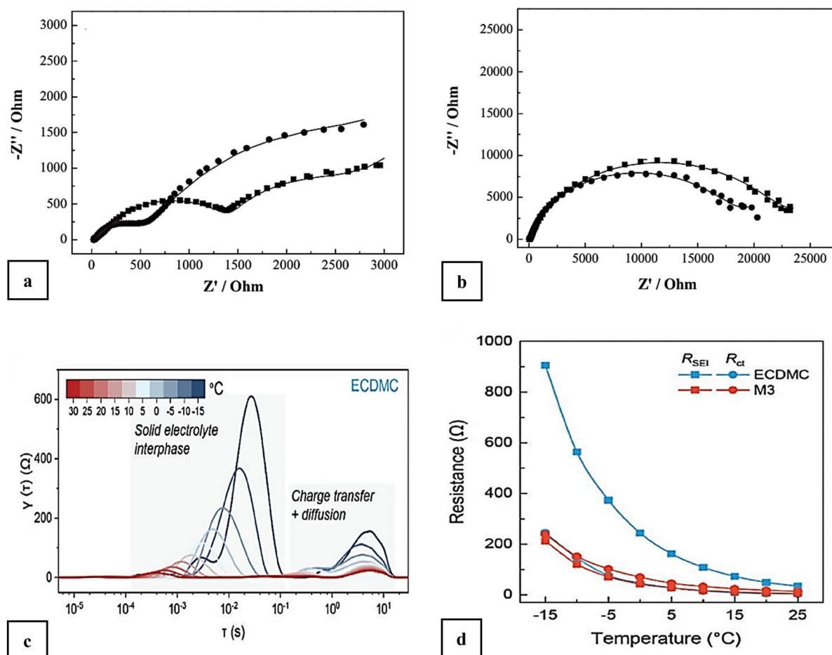
Fig. 6 EIS spectra of delithiated Li/MCMB cells using 1 M \text{LiPF}_6 in EC/PC/EMC (1:3:8 v/v/v) with fluoroethylene carbonate (FEC, squares) and without FEC (circles) at (a) -20\text{ }^\circ\text{C} and (b) -40\text{ }^\circ\text{C} . Reproduced with permission from ref. 34. (c) DRT analysis of the Nyquist plots for graphite electrodes at various temperatures using 1 M \text{LiPF}_6 in EC/DMC (3:7 v/v) electrolyte. Reproduced with permission from ref. 27. (d) R_{\text{SEI}} and R_{\text{ct}} values of graphite electrodes obtained from EIS fitting at different temperatures using various electrolytes. Reproduced with permission from ref. 27.
