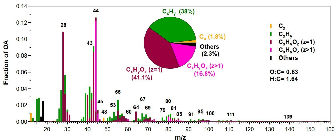
Figure 8. HR mass spectrum of the SOA factor. The most important characteristic m/z ratios were 44, 45, 48, 53, 55, 64, 67, 69, 77, 79, 80, 81, 82, 85, 91, 95, 100, and 111.
