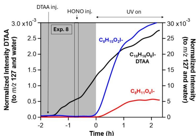
Figure 9. CIMS time-series of DTAA (left y-axis) and products (right y-axis) for exp# 8.
