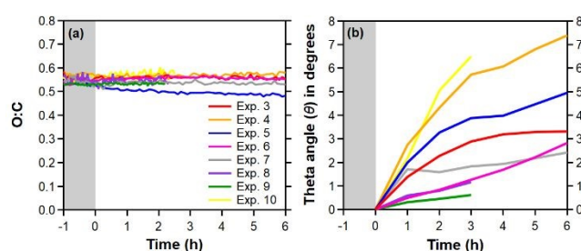
Figure 5. The (a) O:C ratio for the aging experiments and (b) theta ( \theta ) angles of the HR OA spectra for Experiments 3–10.
