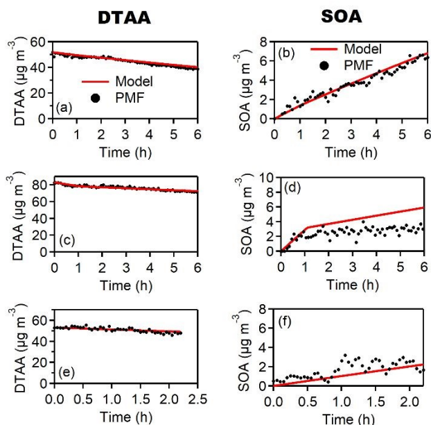
Figure 10. Comparison of model predictions (red line) and experimental measurements (black dots) (in \mu\text{g m}^{-3} ) for three representative oxidation experiments: (a–b) Experiment 6 (low- \text{NO}_x , FORTH-ASC), (c–d) Experiment 7 (high- \text{NO}_x , FORTH-ASC), and (e–f) Experiment 9 (high- \text{NO}_x , CMU-ASC). Panels show pure DTAA and secondary organic aerosol (SOA) formation over time.
