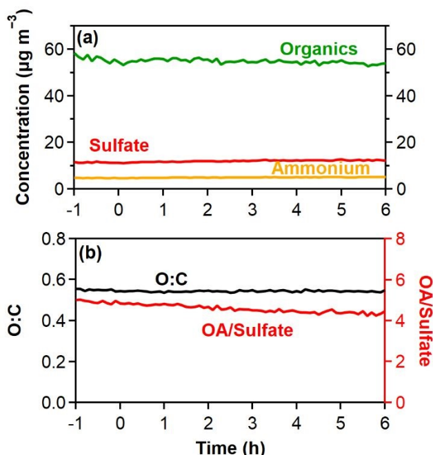
Figure 3. The particle wall-loss corrected (a) mass concentration of OA, sulfate and ammonium in \mu\text{g m}^{-3} and (b) the O:C (black line; left y-axis) and OA/Sulfate (red line; right y-axis) for Exp.1.
