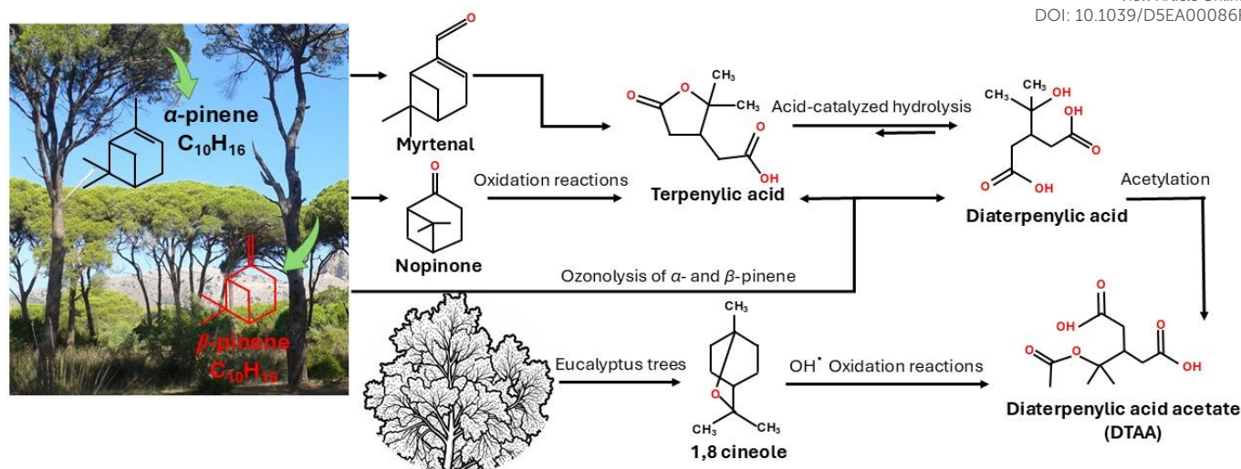
Figure 1. Simplified schematic representation of the reaction pathways leading to the formation of DTAA.
