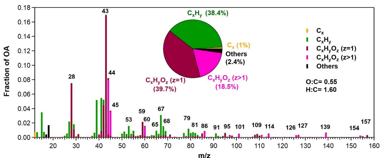
Figure 2. HR average AMS spectrum of pure diaterpenylic acid acetate (DTAA) aerosol. The most important characteristic m/z ratios were 53, 59, 60, 65, 67, 68, 69, 71, 77, 79, 80, 81, 82, 85, 86, 91, 95, 101, 109, 114, 126, 127, 139, 154 and 157.
