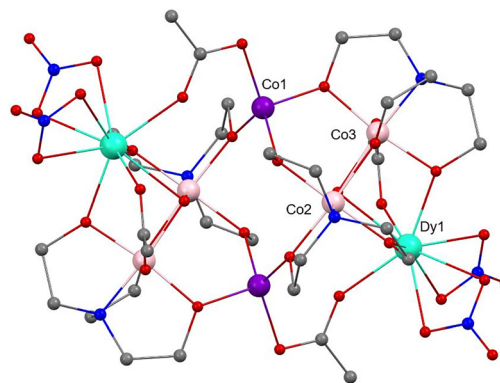
Fig. 1 Ball and stick X-ray structure molecular representation of complex 1 . Hydrogen atoms as well as atoms of disorder components have been omitted for sake of clarity. Co(III): pink; Co(II): violet; Dy: green; O: red; N: blue; C: gray.
