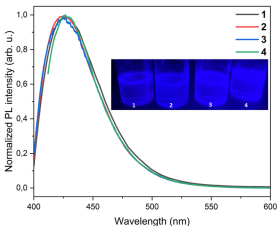
Fig. 4 Emission spectra of the complexes 1–4 (100 \mu\text{M} ) in DMSO, \lambda_{\text{exc}} = 365 \text{ nm} . Inset: photographs of DMSO solutions of complexes 1–4 when excited with 365 nm light. 48
