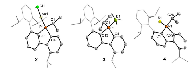
Fig. 1 Molecular structures of 2 (left), 3 (middle) and 4 (right). Ellipsoids drawn at 50% with C–H-atoms omitted, Dipp- and one of the i Pr-groups rendered as wire-frame for clarity. Selected bond lengths [Å] and angles [°] of 2 : C1–P1 1.845(2), C4–P1 1.798(2), C13–P1 1.805(2), P1–Au1 2.2247(6), C11–Au1 2.2885(6); C4–P1–C13 91.83(10), C4–P1–C1 106.46 (10), C13–P1–C1 105.84(10), C4–P1–Au1 114.61(7), C13–P1–Au1 121.62 (7), C1–P1–Au1 113.71(8); C5–C4–P1–C13 179.9(2). 3 : P1–C4 1.7991(13), P1–C13 1.8102(13), P1–C1 1.8435(14), P1–B1 1.9269(16); C4–P1–C13 91.52(6), C4–P1–C1 108.29(6), C13–P1–C1 107.20(6), C4–P1–B1 111.38 (7), C13–P1–B1 121.08(6), C1–P1–B1 114.62(7); C13–P1–C4–C9–178.84 (12); 4 : C20–P1 1.809(1), P1–C20 1.797(1), P1–C28 1.866(1), P1–S1 1.9462 (5); C20–P1–C1 91.78(6), C20–P1–C28 106.39(6), C1–P1–C28 104.83 (6), C28–P1–S1 112.84(5); C20–P1–C1–C2 175.58(12).
