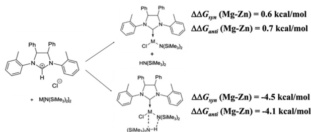
Scheme 2 Free energy difference in benzene as a solvent, calculated for the formation of monomeric complexes of M = Zn and Mg ( \Delta\Delta G_{syn} (Mg-Zn) and \Delta\Delta G_{anti} (Mg-Zn), respectively) with the reactants and reaction products at an infinite distance.
