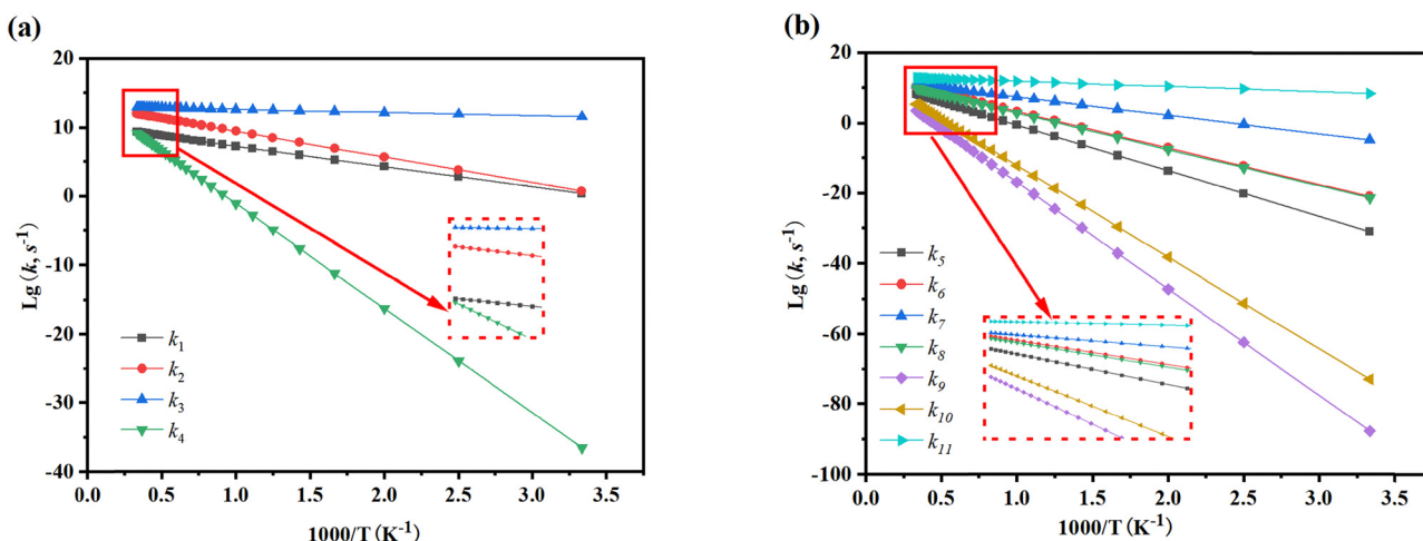
Fig. 9 (a) Reaction rate constant diagrams for the \text{AlO}/\text{HF} system. (b) Reaction rate constant diagrams for the \text{Al}_2\text{O}_3/\text{HF} system.
