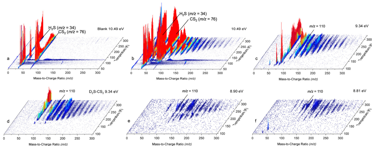
Fig. 5 PI-ReToF-MS spectra recorded during the TPD of hydrogen sulfide–carbon disulfide ices: unirradiated (blank) \text{H}_2\text{S-CS}_2 ice recorded at 10.49 eV (a), the irradiated \text{H}_2\text{S-CS}_2 ice recorded at 10.49 (b), 9.34 (c), 8.90 (e), and 8.81 eV (f), and the irradiated \text{D}_2\text{S-CS}_2 ice recorded at 9.34 eV (d).
