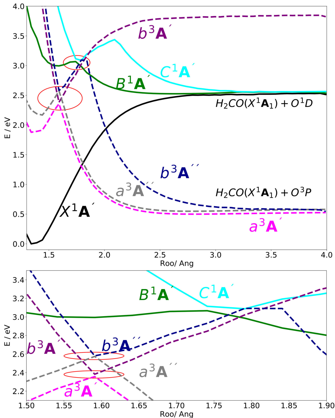
Fig. 19 (Upper) the adiabatic PE curves along the \text{OO} stretching mode for the X^1A' , B^1A' , C^1A' , a^3A' , b^3A' , a^3A'' and b^3A'' states. (Lower) the adiabatic PE curves along \text{O}-\text{O} stretching mode, zooming in geometries in the range 1.55 < R_{\text{OO}} < 1.80 (indicated by red circles in the upper panel). The bonding angle \theta_{\text{COO}} and the stretching mode R_{\text{CO}} are fixed at the equilibrium structure values 117.905^\circ and 1.27 , respectively.
