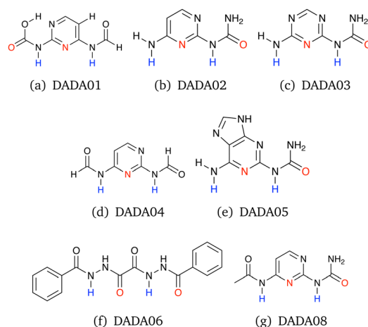
Fig. 1 The monomers of the quadruply hydrogen-bonded dimers with DADA–ADAD hydrogen-bonding pattern. The previously studied DADA07 1 is omitted because the CCSD(T)-cf reference data are not available. The figures are made with Jmol. 52
