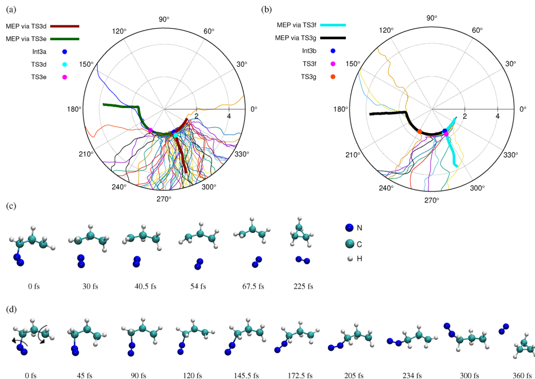
Fig. 7 Plots of \angle \text{C1–C2–C3–N4} versus C3–N4 for the minimum energy path, all stationary points along the minimum energy path, and the TS3a trajectories that dissociate from the (a) Int3a and (b) Int3b . (c) Snapshots of a sample trajectory in which the C3–N4 bond dissociates in the TS3a region of the PES. (d) Snapshots of a trajectory in which the \text{N}_2 group rotates 273 around the C3–N4 bond before dissociating via the S_{\text{H}2} -like transition state TS3g .
