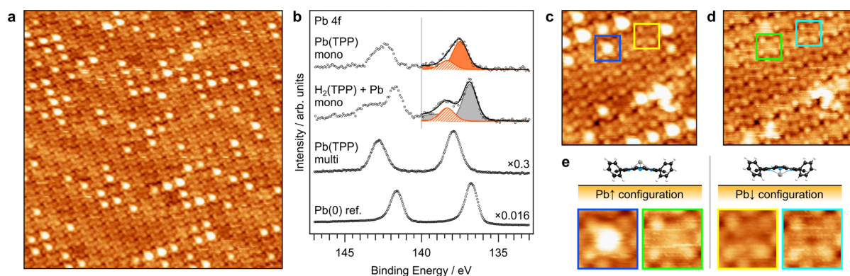
Fig. 2 (a) STM image of a \text{Pb}(\text{TPP}) monolayer showing an ordered adsorbate structure in which two adsorption configurations ( \text{Pb}\uparrow and \text{Pb}\downarrow ) coexists. (b) Pb 4f spectra of a directly deposited \text{Pb}(\text{TPP}) monolayer, a partially metalated \text{H}_2(\text{TPP}) monolayer by deposition of Pb atoms, a \text{Pb}(\text{TPP}) multilayer, and a \text{Pb}(0) reference on \text{Au}(111) . The Pb 4f_{7/2} region of the monolayer spectra is described by a fit function of \text{Pb}(\text{TPP}) colored in orange with the \text{Pb}\uparrow isomer shown hatched as well as the signal of unreacted \text{Pb}(0) atoms colored in gray. (c,d) STM images of the same surface are, scanned with negative (left) and positive (right) bias voltage. \text{Pb}\uparrow and \text{Pb}\downarrow configurations show different appearances depending on the tunneling bias. (e) Image sections from (c), (d) showing the \text{Pb}\uparrow and \text{Pb}\downarrow isomers. Tunneling parameters and image size: (a) U = -1.20 \text{ V} , I = -0.16 \text{ nA} , 30 \times 30 \text{ nm}^2 ; (c) U = -1.20 \text{ V} , I = -0.09 \text{ nA} , 10 \times 10 \text{ nm}^2 ; (d) U = +1.20 \text{ V} , I = +0.09 \text{ nA} , 10 \times 10 \text{ nm}^2 , (e) U = +1.20 \text{ V} , I = +0.09 \text{ nA} , 1.8 \times 1.8 \text{ nm}^2 .
