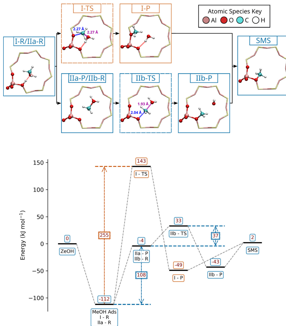
Fig. 2 Energy profile for SMS formation proceeding via CH 3 OH on H-SSZ-13. The energies are shown for the reactants (R), products (P), and transition states (TS) of reactions (I) and (II). The route with the highest barrier is shown in orange, and the lowest barrier in blue. Energies are referenced to the isolated Brønsted acid site of H-SSZ-13. All calculations were performed with PBE-MBD. The annotated transition states structures are shown for reactions (I) and (IIb).
