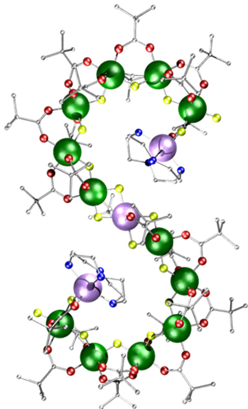
Fig. 1 Crystal structure of [\text{Ni}(\text{cyclen})]_2\text{Cr}_{12}\text{NiF}_{18}(\text{O}_2\text{C}^t\text{Bu})_{24} 1 (where cyclen = 1,4,7,10-tetracyclododecane). Colours: Cr, green; Ni, purple; F, yellow; O, red; N, blue; C, grey. Hydrogen atoms are omitted for clarity.
