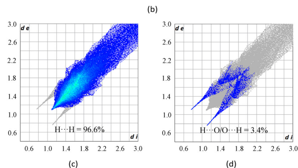
Fig. 4 Hirshfeld surfaces mapped with d_{\text{norm}} for (a) the asymmetric unit and (b) the six molecular clusters of SOF-1 . Intermolecular interactions at the sum of the vdW contacts are highlighted in white, while shorter and longer contacts are represented in red and blue, respectively. Two-dimensional fingerprint plots for the (c) H⋯H and (d) H⋯O/O⋯H contacts of SOF-1 .
