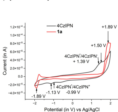
Fig. 1 Mechanistic studies. (a) Control experiments. (b) UV-visible spectra showing 4CzIPN as the sole absorbing species under 427 nm irradiation. (c) Luminescence quenching of a 10 −4 M solution of 4CzIPN by 1a . (d) Stern–Volmer plot. (e) Cyclic voltammograms of 4CzIPN and 1a to validate the proposed triplet energy transfer.
