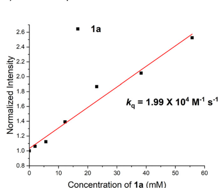
Fig. 1 Mechanistic studies. (a) Control experiments. (b) UV-visible spectra showing 4CzIPN as the sole absorbing species under 427 nm irradiation. (c) Luminescence quenching of a 10 −4 M solution of 4CzIPN by 1a . (d) Stern–Volmer plot. (e) Cyclic voltammograms of 4CzIPN and 1a to validate the proposed triplet energy transfer.
