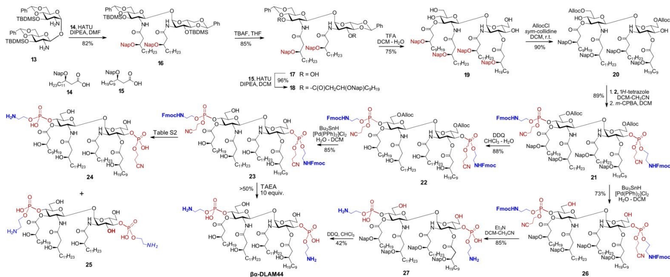
Scheme 2. Synthesis of PE-modified glycolipid \beta\alpha -DLAM44
