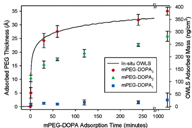
Fig. 5 Time-dependent adsorption of mPEG-DOPA onto \text{TiO}_2 . Reproduced with permission from ref. 27. Copyright 2005 American Chemical Society.
