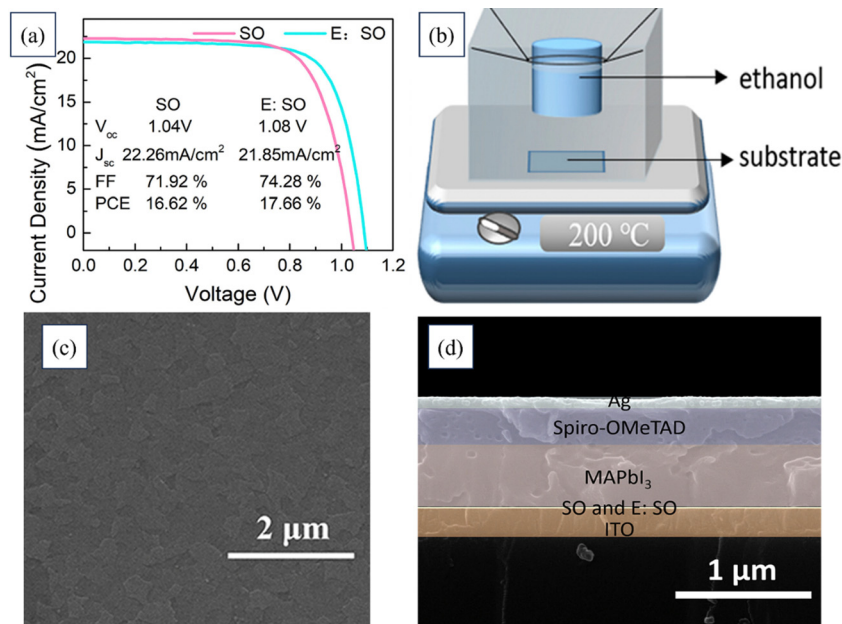
Fig. 23 (a) J-V curves of a device based on the SnO 2 film with and without ethanol vapour treatment. (b) Schematics of the ethanol vapour experimental set-up. SEM images of (c) SnO 2 layer deposited in ethanol vapour and (d) cross-section of the tested device. Reproduced with permission. 202 Copyright 2020, Elsevier.
