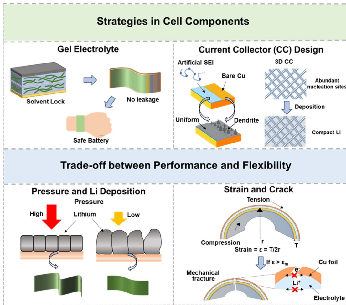
Fig. 16 Potential strategies and critical factors for implementing flexible anode-free lithium metal batteries.
