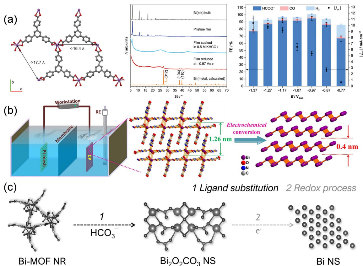
Fig. 12 (a) Structural representation, XRD spectra and FE data of Bi(bt). 52 Copyright 2020, Wiley-VCH. (b) Schematic illustration depicting the preparation of Bi-ene. 111 Copyright 2020, Wiley-VCH. (c) Schematic illustration depicting the in situ reconstruction process of Bi-MOF NRs to Bi NSs. 104 Copyright 2021, Wiley-VCH.
