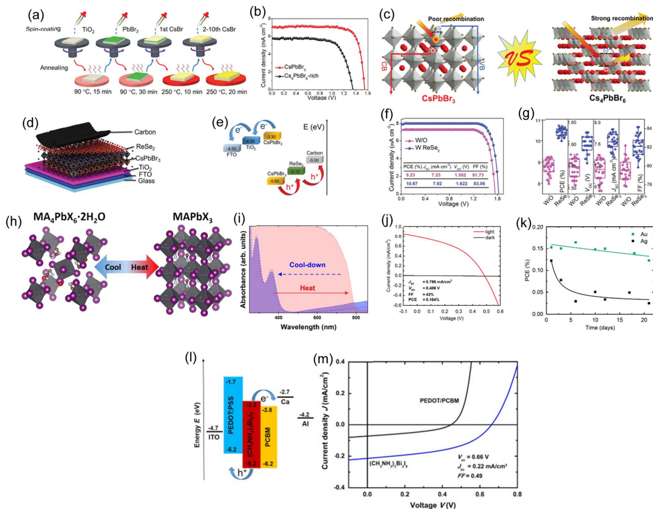
Fig. 2 (a) Schematic of the multi-step production method. (b) The J - V characteristics of \text{CsPbBr}_3 based PSCs with and without \text{Cs}_4\text{PbBr}_6 . (c) The process by which carrier recombination was induced by \text{Cs}_4\text{PbBr}_6 . (d) All-inorganic \text{CsPbBr}_3 PSC with a \text{ReSe}_2 -tailored structure. (e) Energy level of the all-inorganic, \text{ReSe}_2 -tailored \text{CsPbBr}_3 PSC. (f) J - V curves. (g) Statistics of the PVs of different PSCs with and without \text{ReSe}_2 . (a)–(g) Reproduced with permission. 60 Copyright 2022, Wiley. (h) In the top left corner is the crystal structure of \text{MA}_4\text{PbI}_6 \cdot 2\text{H}_2\text{O} , and in the top right corner is \text{MAPbI}_3 . (i) Images illustrate the optical absorption of a pure sample of methylammonium lead iodide (blue), after thermal annealing at 100^\circ\text{C} (red), and after cooling to ambient temperature (blue dashes). (h) and (i) Reproduced with permission. 61 2021, ACS. (j) J - V characteristics. (k) The stability of MABI devices with Ag and Au top contacts is plotted as a PCE with time. (j) and (k) Reproduced with permission. 63 Copyright 2017, RSC. (l) Numbers in the energy level diagram are given in relation to the vacuum. (m) J - V curves for devices with a (\text{CH}_3\text{NH}_3)_3\text{Bi}_2\text{I}_9 absorber (blue) and a reference cell without an absorber (black) under illumination. (l) and (m) Reproduced with permission. 63 Copyright 2016, Elsevier.
