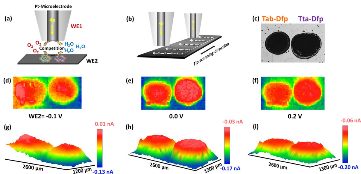
Fig. 4 (a) Schematic representation of RC-SECM mode (WE1: Pt microelectrode and WE2: catalyst coated GC plate), (b) SECM array scan, (c) microscopic images of Tta-Dfp and Tab-Dfp over the GC plate, 2D RC-SECM images of Tta-Dfp and Tab-Dfp spots measured in 400 mM HCl with different applied sample potentials: (d) -0.1 V, (e) 0.0 V, (f) 0.2 V and (g-i) their corresponding 3D images respectively. The tip (Pt-microelectrode) was polarized at 0.2 V.
