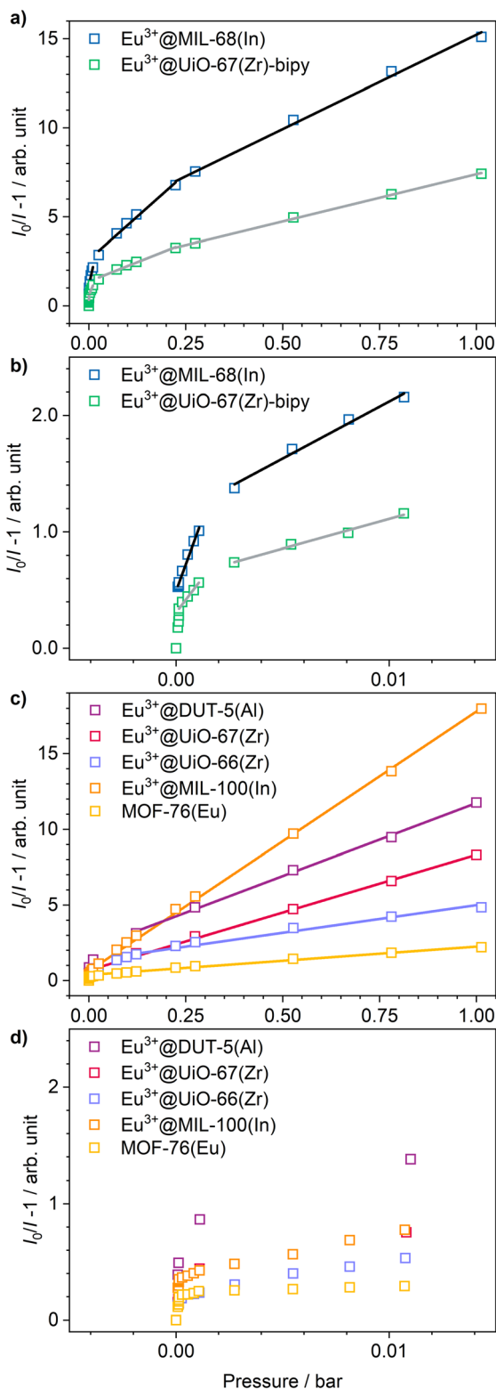
Fig. 7 Stern–Volmer plots and fits of Eu 3+ @MIL-68(In) and Eu 3+ @UiO-67(Zr)-bipy. (a) Full pressure range, (b) enlarged view of points collected at lower pressures. All other impregnated MOFs are shown in (c) and (d), respectively.
