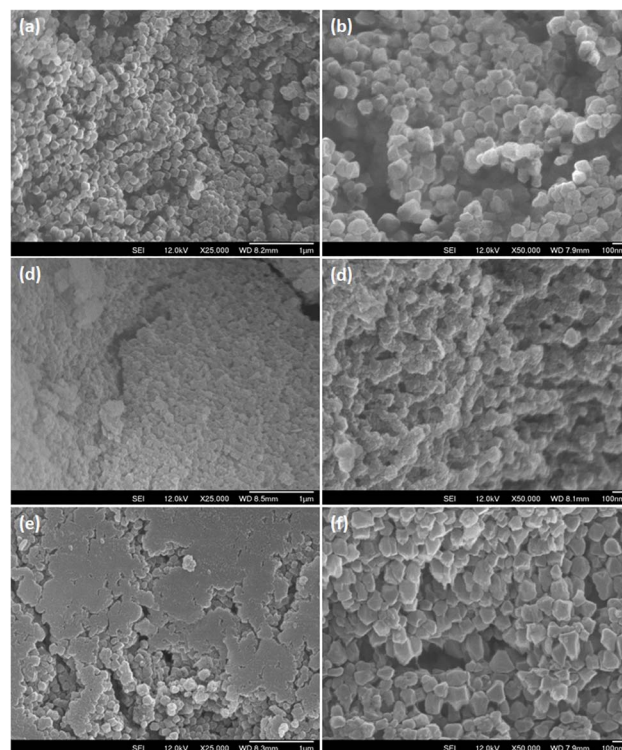
Fig. 13 FESEM images of MIL-101(Cr)/polymer coatings: 3MIL-101(Cr)/1PVA coating with scale bars at (a) 1\ \mu\text{m} and (b) 100\ \text{nm} , the 2MIL-101(Cr)/1silicate coating with scale bars at (c) 1\ \mu\text{m} and (d) 100\ \text{nm} and the 3MIL-101(Cr)/1HEC coating with scale bars at (e) 1\ \mu\text{m} and (f) 100\ \text{nm} .
