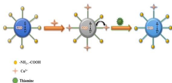
Fig. 10 Fluorescence quenching of CQDs by \text{Cu}^{2+} following the PET mechanism and the recovery of fluorescence after adding thiamine. 98
